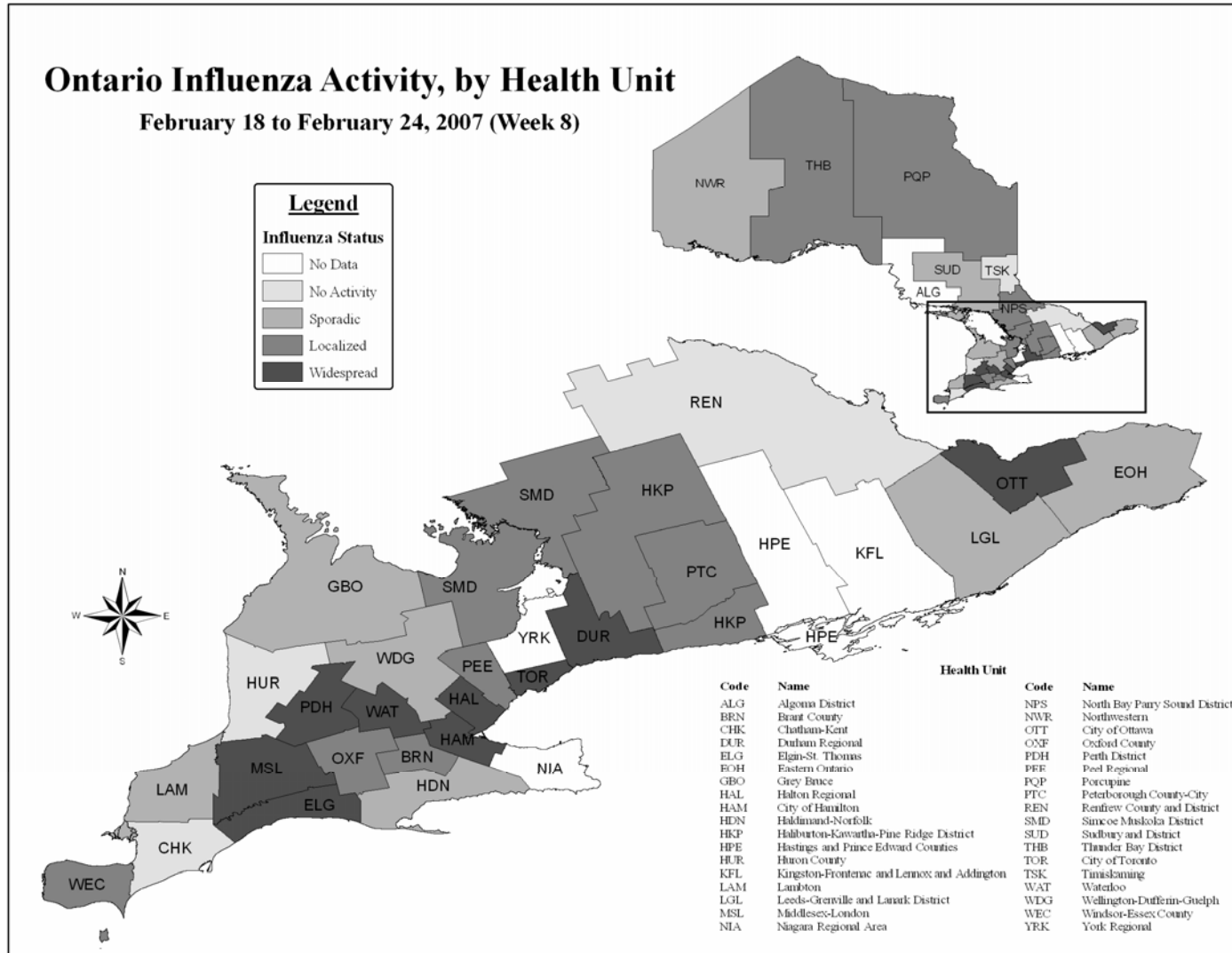
Figure 3: Influenza Activity* levels in Ontario by health unit & health region for Week 8.
