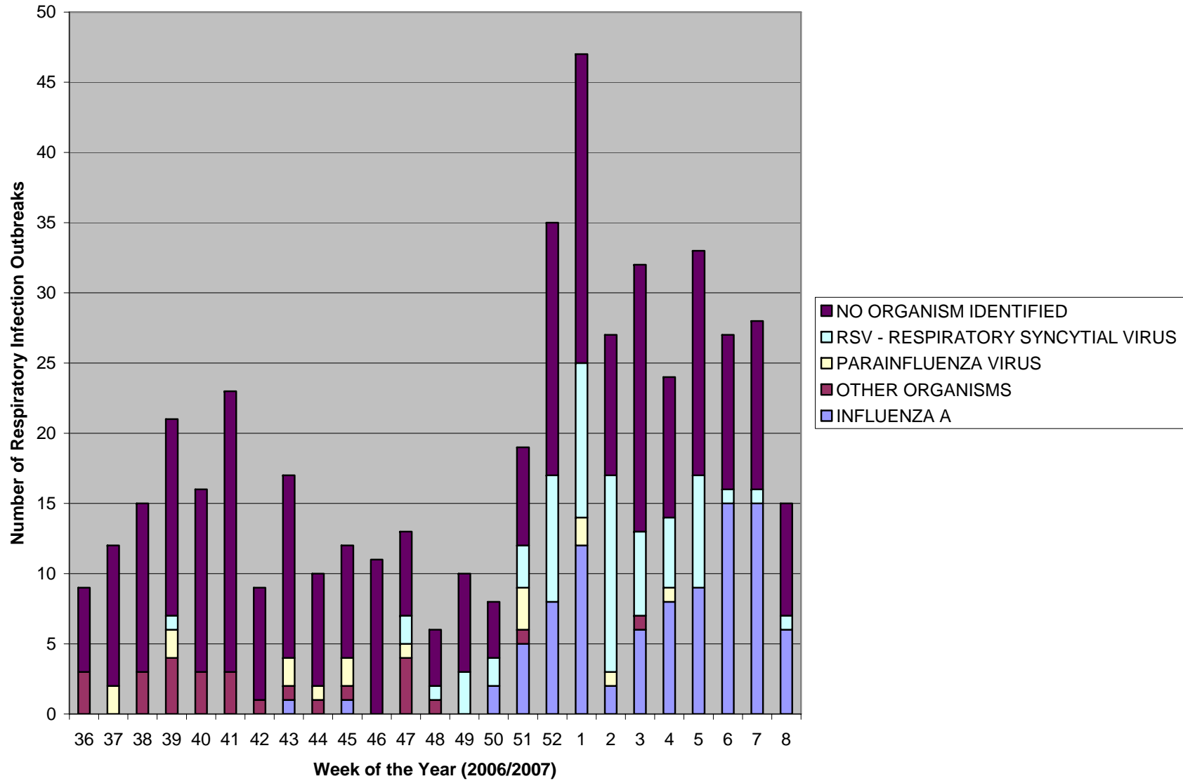
Figure 2: Institutional respiratory infection outbreaks in Ontario by onset of illness in the first case: Total Outbreaks from September 1, 2006 – February 24, 2007 by causative organism
